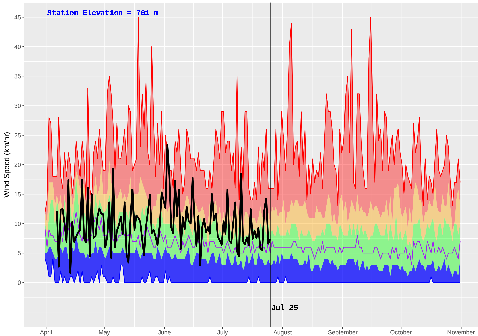
HORSEFLY (230) : Historical (1971–2016) and Current (2017) Noon Wind Speed
